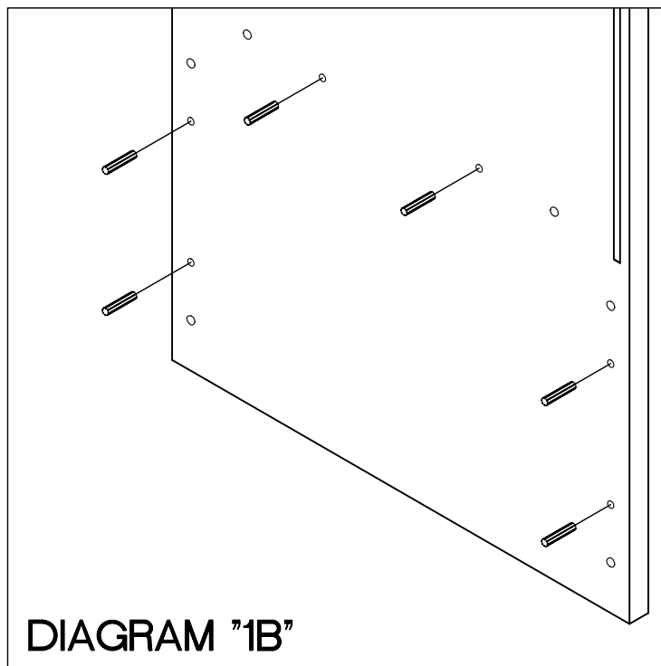
TYP. END PANEL (RIGHT END SHOWN)
